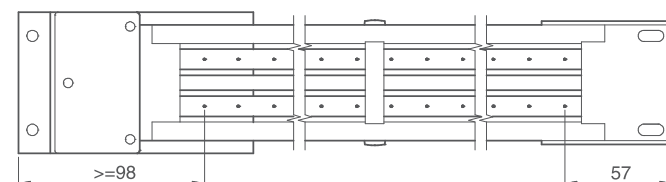
Technical drawing P-Sh-N-Ex
